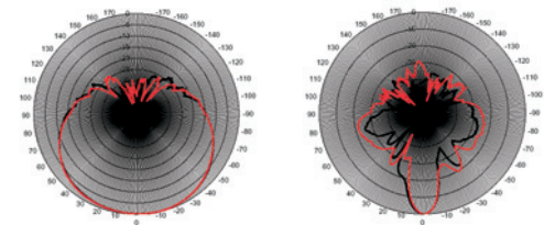
Radiation patterns PRO-SECTOR50016V_BOX
